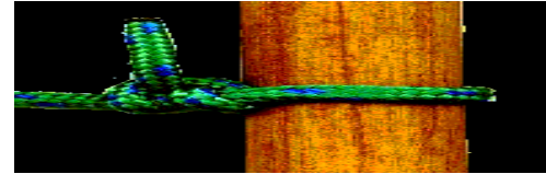
Two Half Hitches Used to attach a rope to a pole or guy point. Must be securely tightened.
